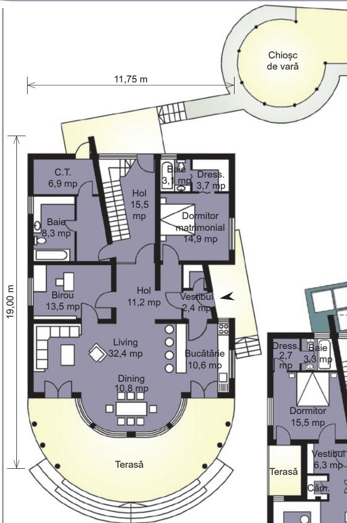
PLAN PARTER
