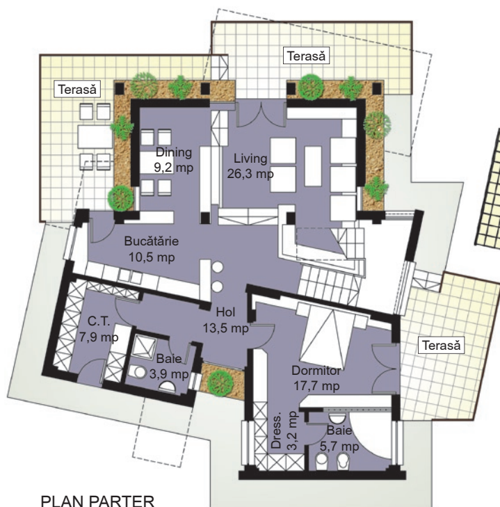
PLAN PARTER
