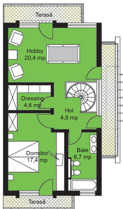
PLAN MANSARDĂ
